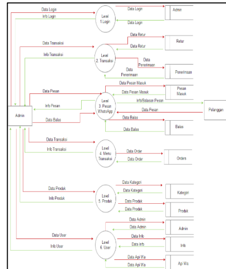
Gambar 6. DFD Level 1.
